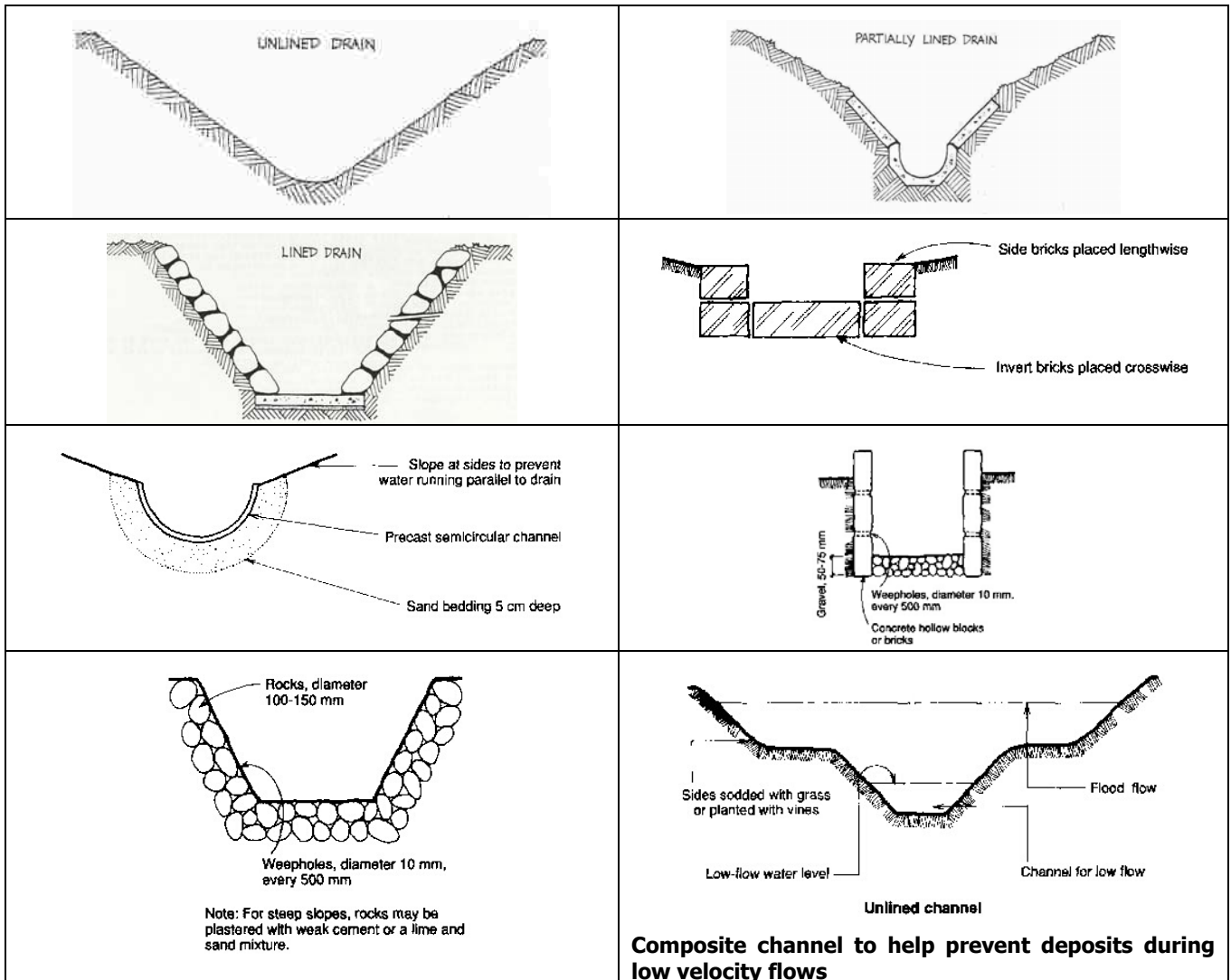
Variations in simple drainage cross-sections (Refs: taken directly from UNCHS (Habitat), 1986; WHO, 1991)
