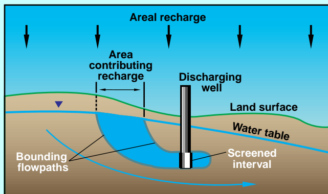
Figure 1. Area contributing recharge to a single discharging well in a simplified hypothetical ground-water system.
