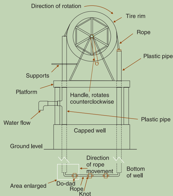
Front view of Rope Pump
