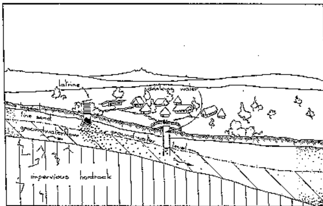
Figure 4: Contamination of wells from pit latrines
