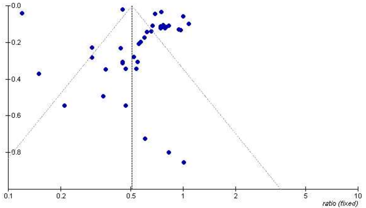
Figure 01. Funnel plot to explore publication bias
